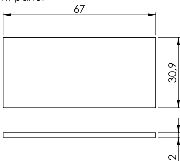
Front panel
