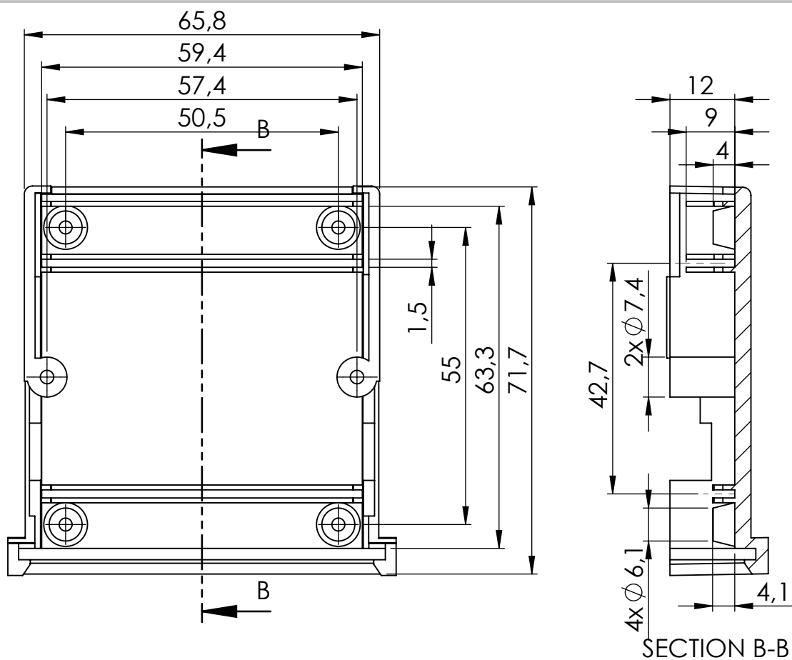
Rear panel
