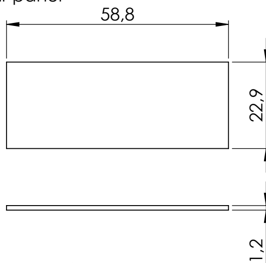
Rear panel
